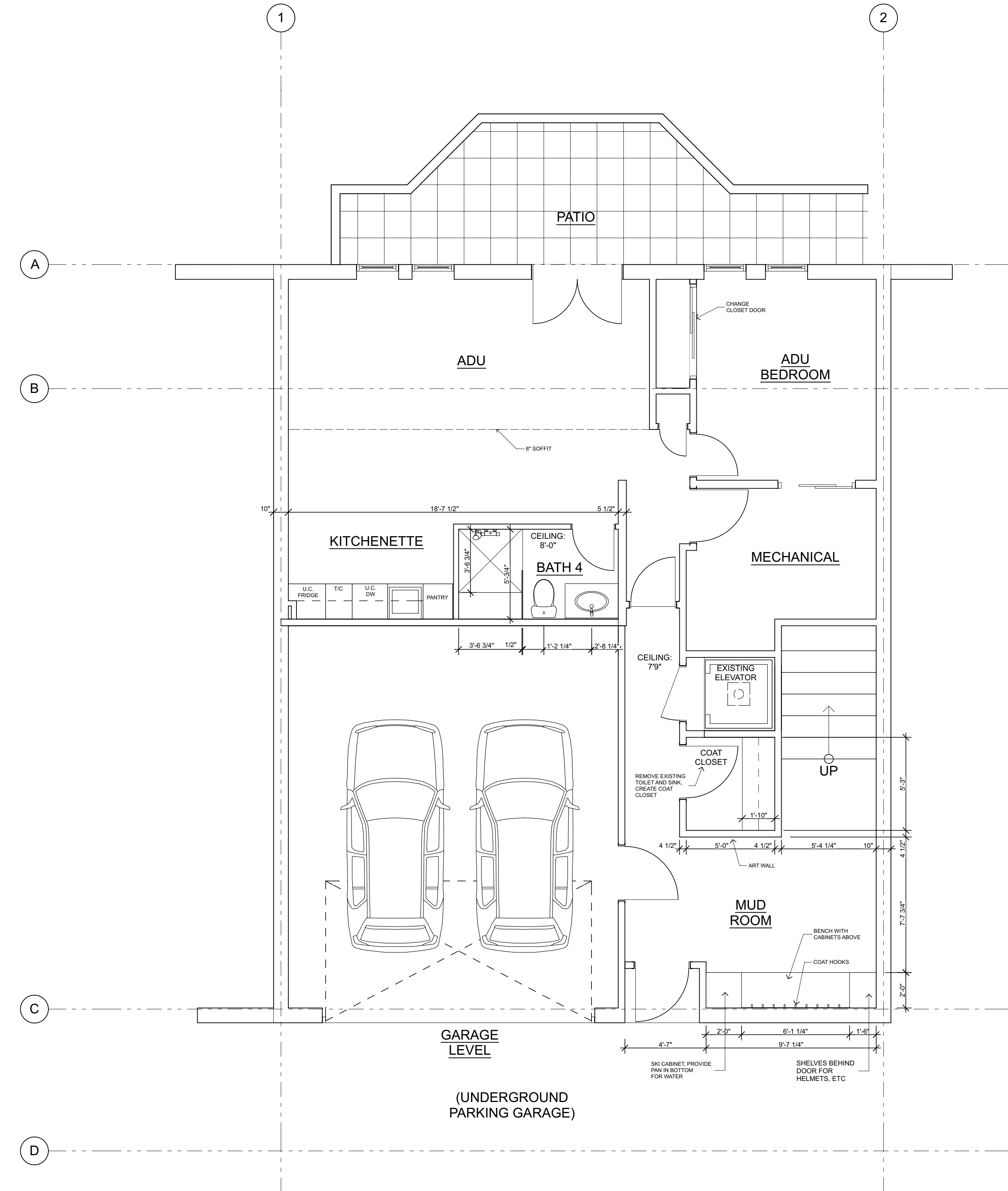
2 PROPOSED - GARAGE LEVEL SCALE: 1/4" = 1'-0"
