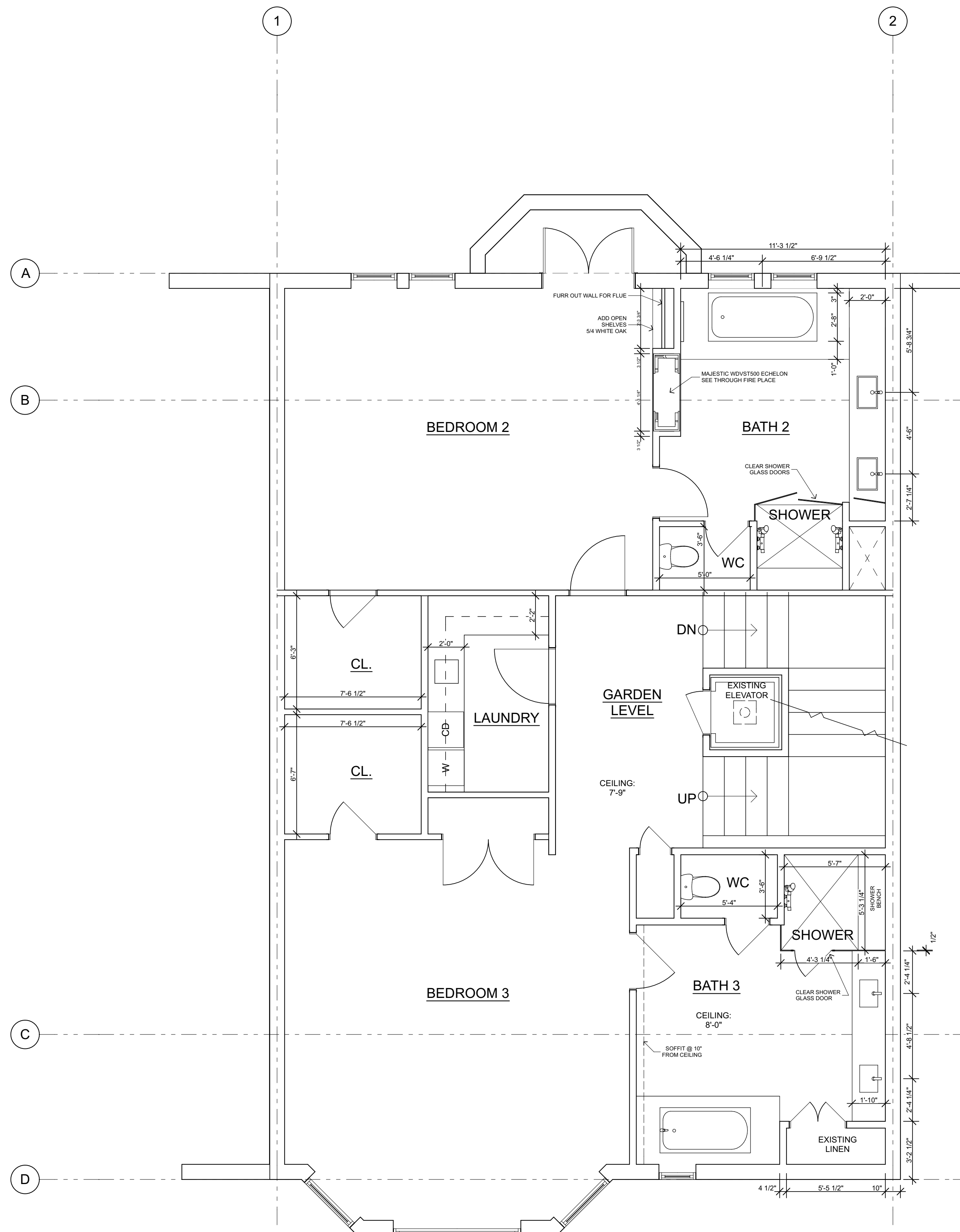
1 PROPOSED - GARDEN LEVEL SCALE: 1/4" = 1'-0"
