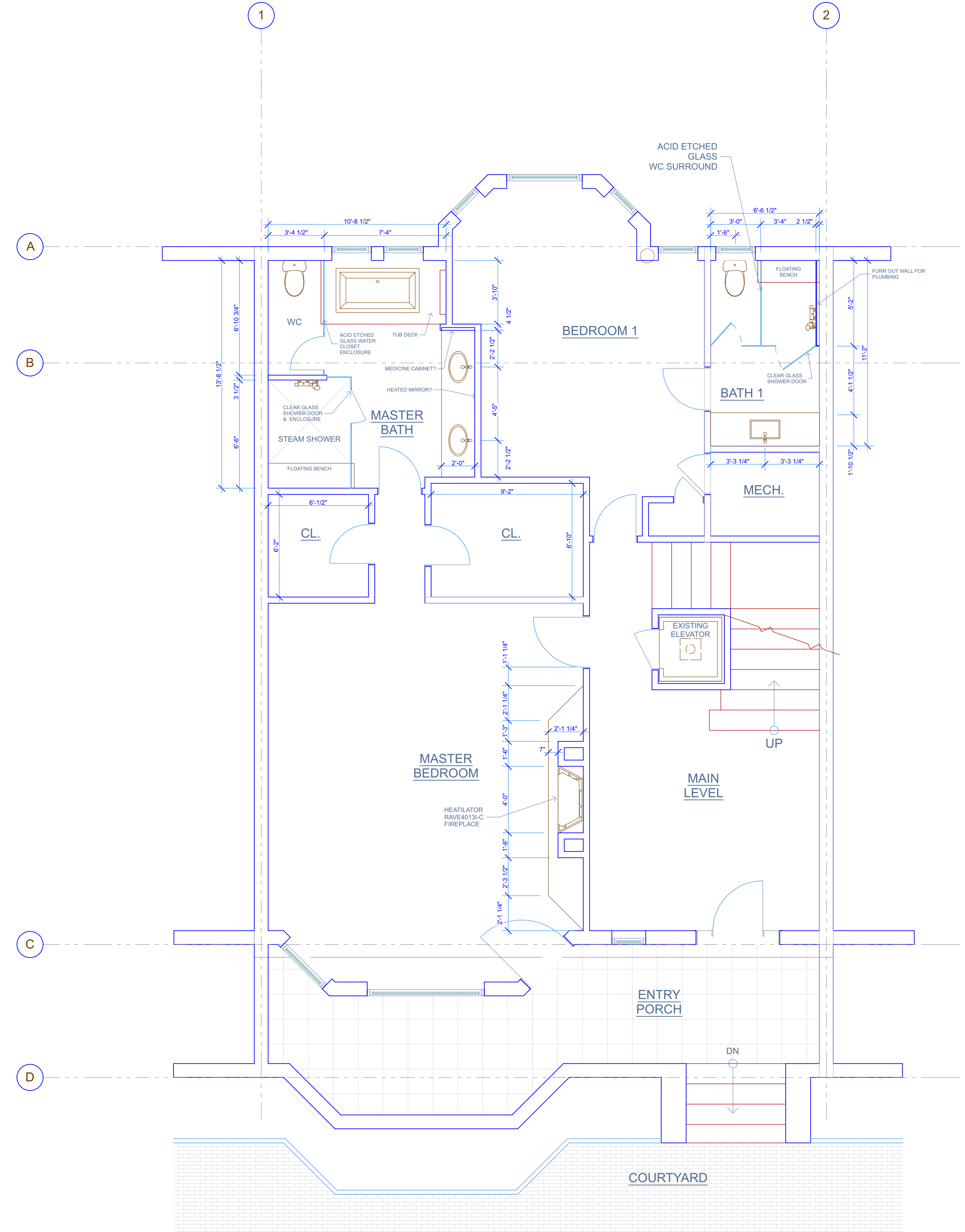
2 PROPOSED - MAIN ENTRY LEVEL SCALE: 1/4" = 1'-0"
